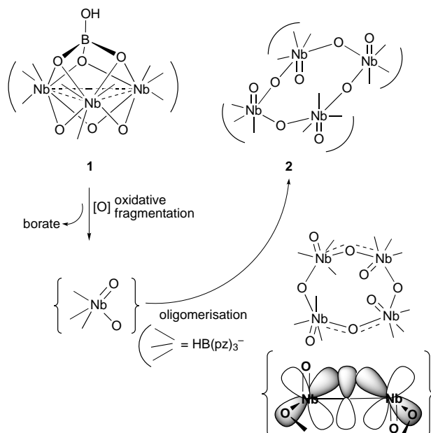
Scheme 2 Reactions leading to the formation of complex 2 from 1 . Inset: linear Nb 4d_\pi O p_\pi bonding in the tetrameric core
